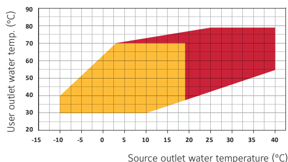
Operation limits
