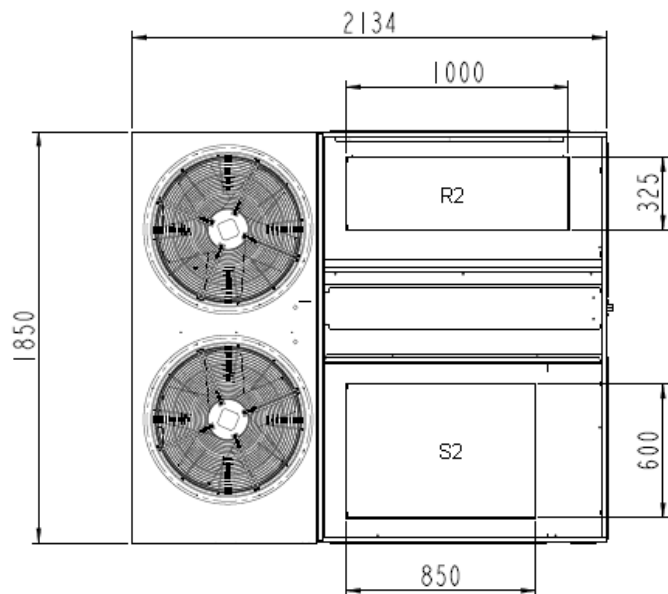
TOP VIEW WITHOUT ROOF PANEL
