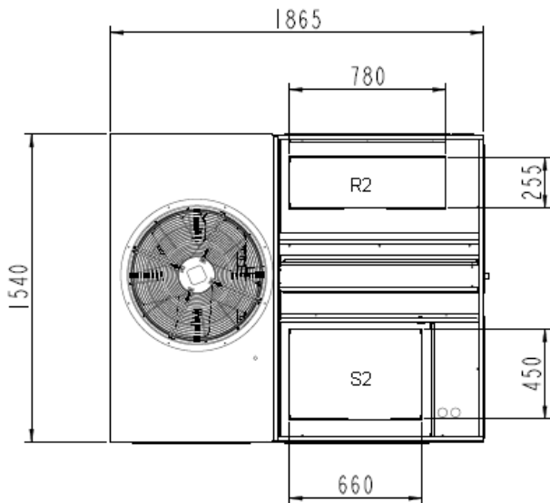
TOP VIEW WITHOUT ROOF PANEL
