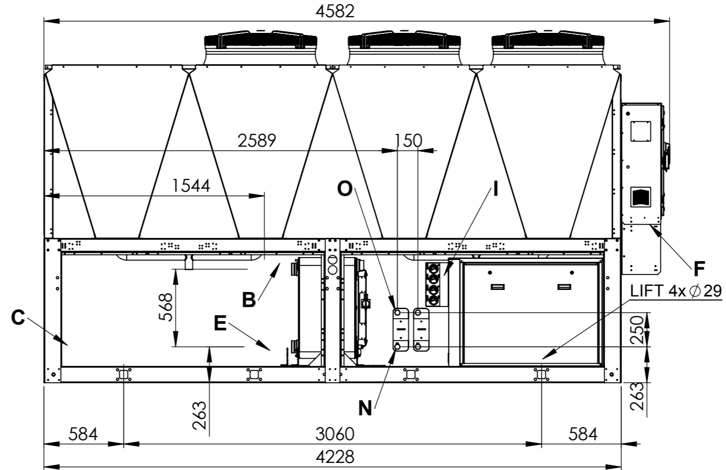
VISTA LATERALE SIDE VIEW
