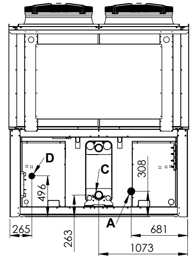
VISTA POSTERIORE BACK VIEW
