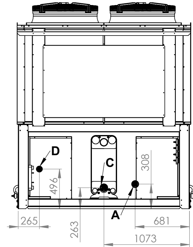
VISTA POSTERIORE BACK VIEW
